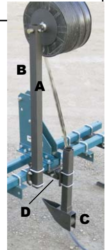
Drip Tape Application
